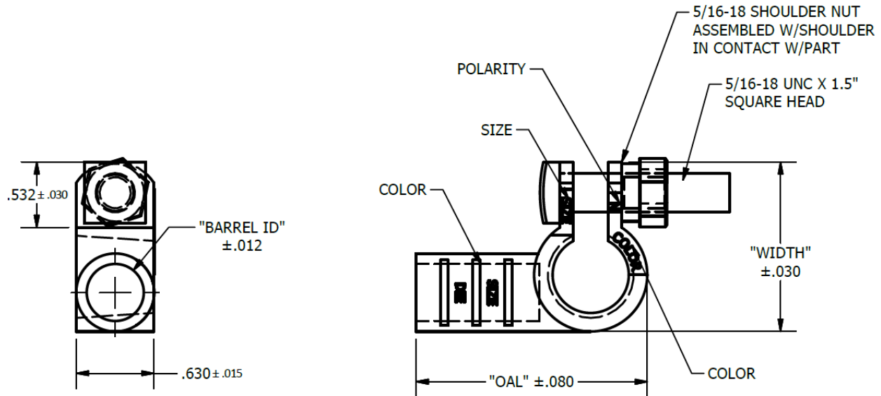
Pictured is a Left Elbow Terminal
